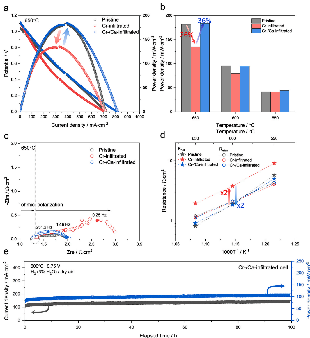
Fig. 4. (a) Typical I-V-P curves of the pristine, Cr-infiltrated and Cr-/Ca-infiltrated single cells at 650 °C under wet H 2 at the anode and the air at the cathode. Note that I denotes the current density, V is the potential, and P is the power density. (b) Comparison of the resulting peak power densities between the cells at T = 550 –650 °C. (c) Impedance spectra of three different cells at 650 °C. (d) Temperature dependence of resistance values corresponding to the ohmic ( R_{ohm} ) and polarization ( R_{pol} ) resistance, respectively. (e) Long-term stability test of the single cell with Cr-/Ca-infiltrated PCO cathode for 100 h measured at 650 °C under a constant voltage of 0.75 V.
