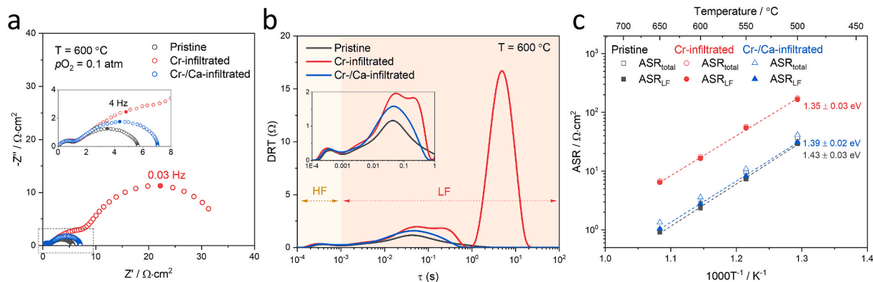
Fig. 1. (a) Typical impedance spectra and (b) distribution of relaxation time (DRT) plots of the PCO/YSZ/PCO symmetric cells (pristine and with serial infiltration of Cr- and Ca-additives) measured at 600 °C. (c) Arrhenius plot of the total (ASR total ) and LF (ASR LF ) polarization resistances.
