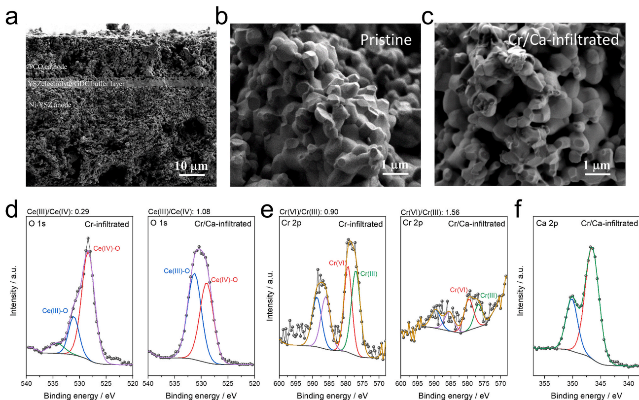
Fig. 2. (a) Cross-sectional SEM image of a Ni-YSZ/YSZ/GDC/PCO anode-supported single cell. Magnified SEM images of (b) the pristine and (c) the Cr-/Ca-infiltrated PCO cathode after fuel cell measurements. Comparison of XPS spectra of (d) O 1s and (e) Cr 2p for the Cr-infiltrated and Cr/Ca-infiltrated single cells. XPS spectra of (f) Ca 2p for the Cr/Ca-infiltrated single cell.
