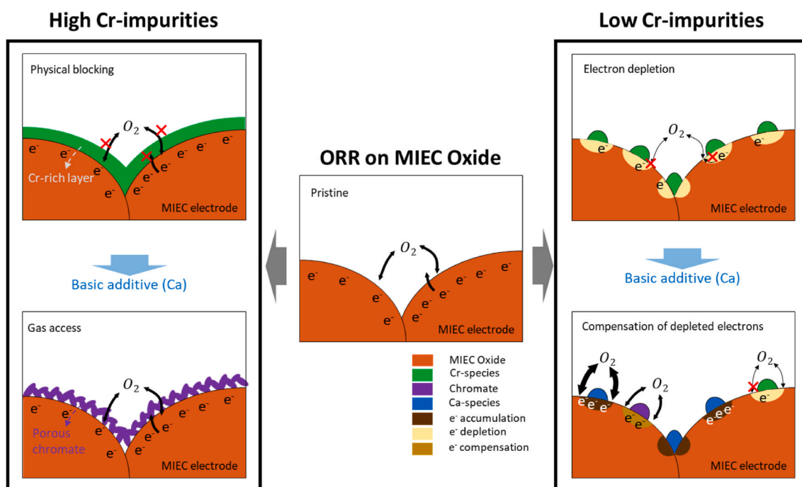
Fig. 3. Schematic illustration of Cr-poisoning mechanisms at different concentration levels and the strategy to achieve recovery by subsequent infiltration with CaO species. See text for further discussion.
